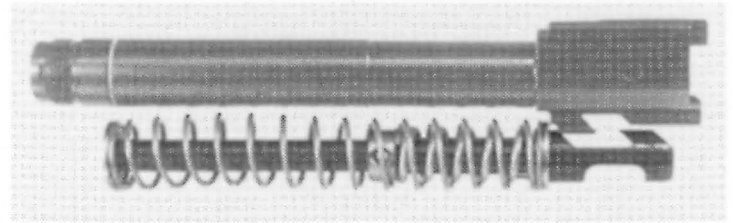
Lage Pufferstange
